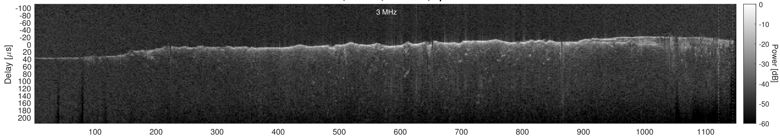
Orbit 11088, Cluttergram
