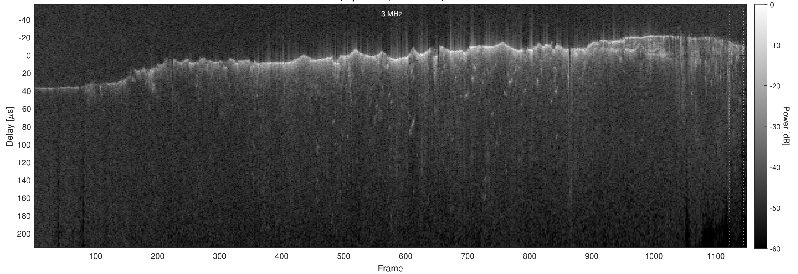
Orbit 11088, Optimized, No Window, Channel 2
