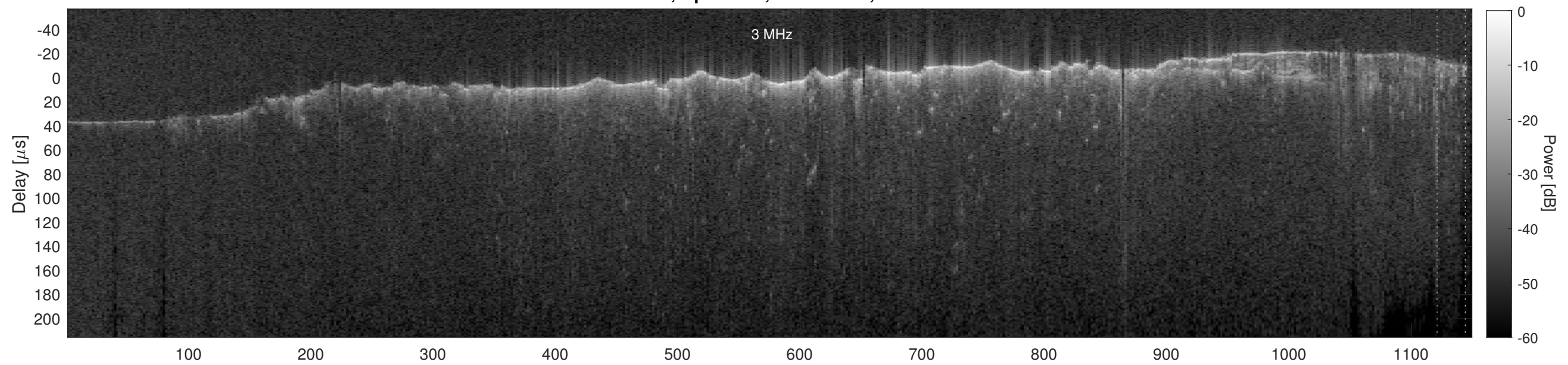
Orbit 11088, Cluttergram
