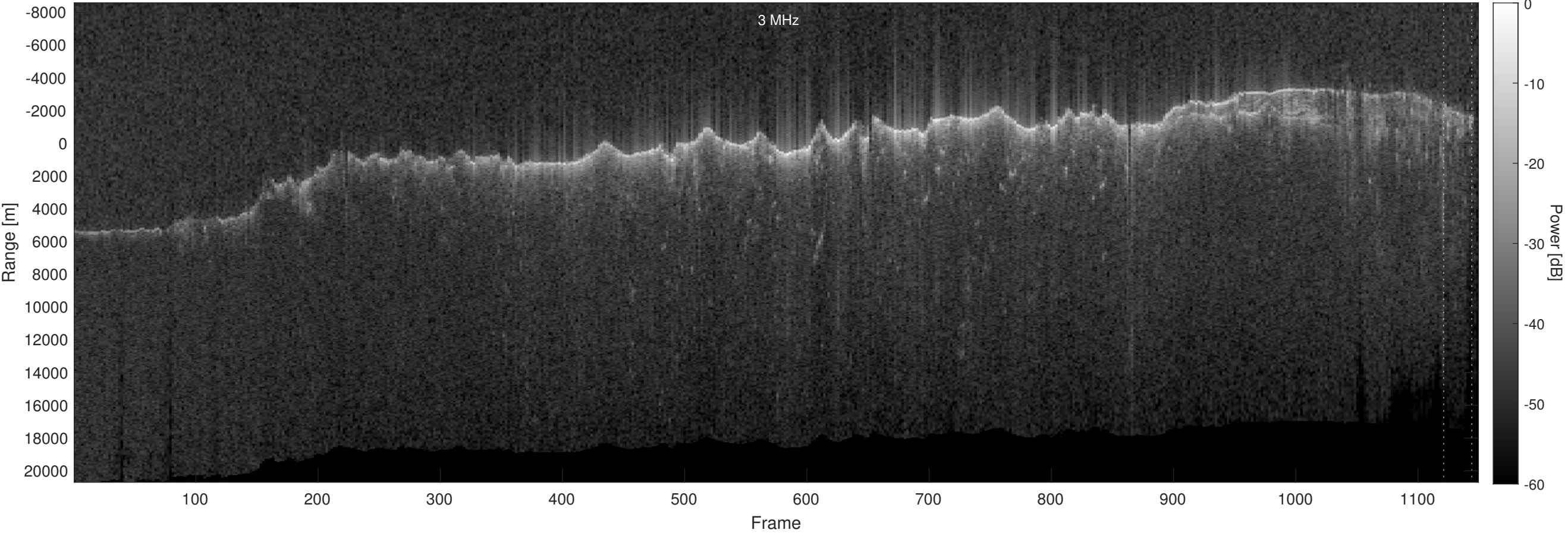
Orbit 11088, Optimized, No Window, Depth-Corrected, Channel 2
