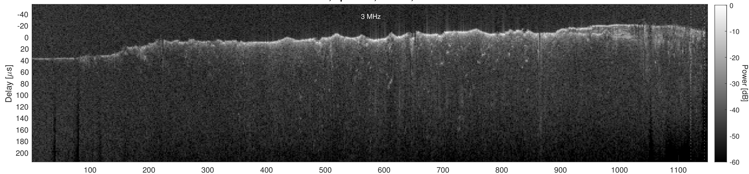
Orbit 11088, Cluttergram
