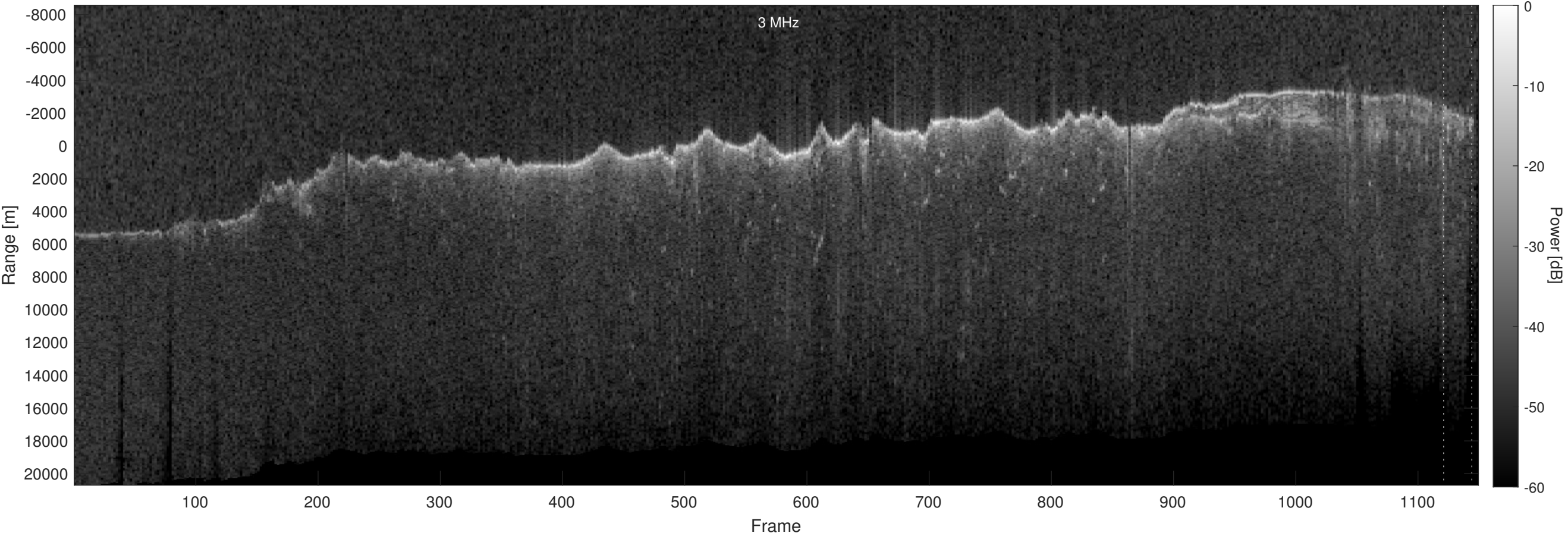
Orbit 11088, Optimized, Window, Depth-Corrected, Channel 2
