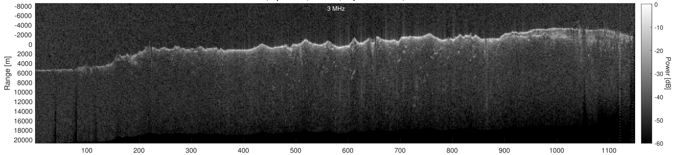
Orbit 11088, Depth-Corrected Cluttergram
