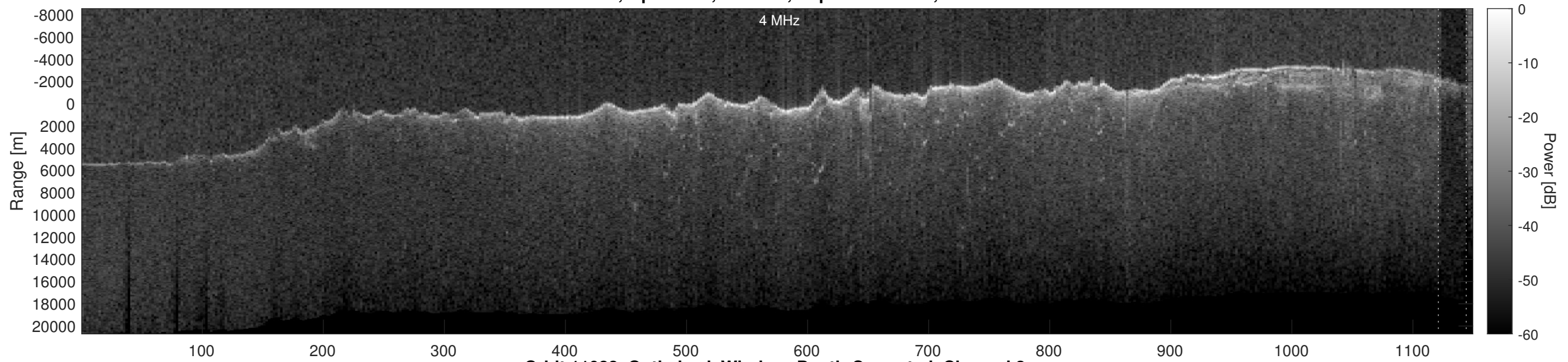
Orbit 11088, Optimized, Window, Depth-Corrected, Channel 2
