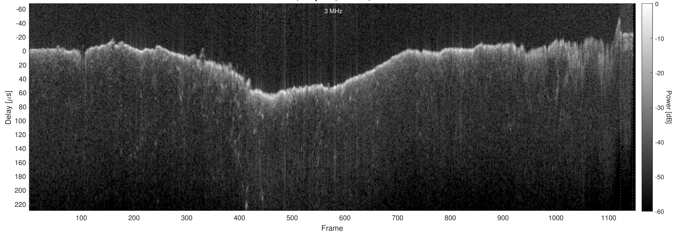
Orbit 11089, Chapman, Window, Channel 2
