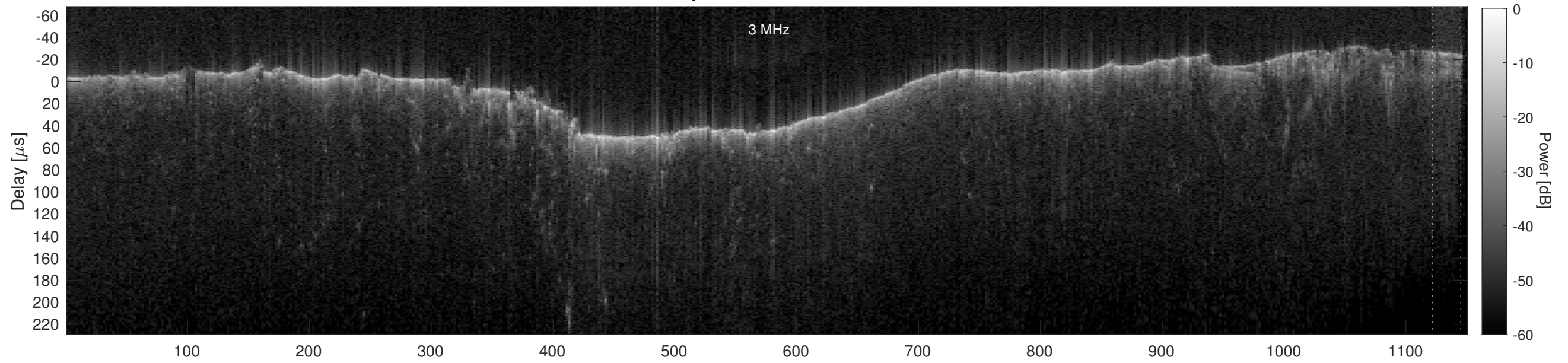
Orbit 11089, Cluttergram
