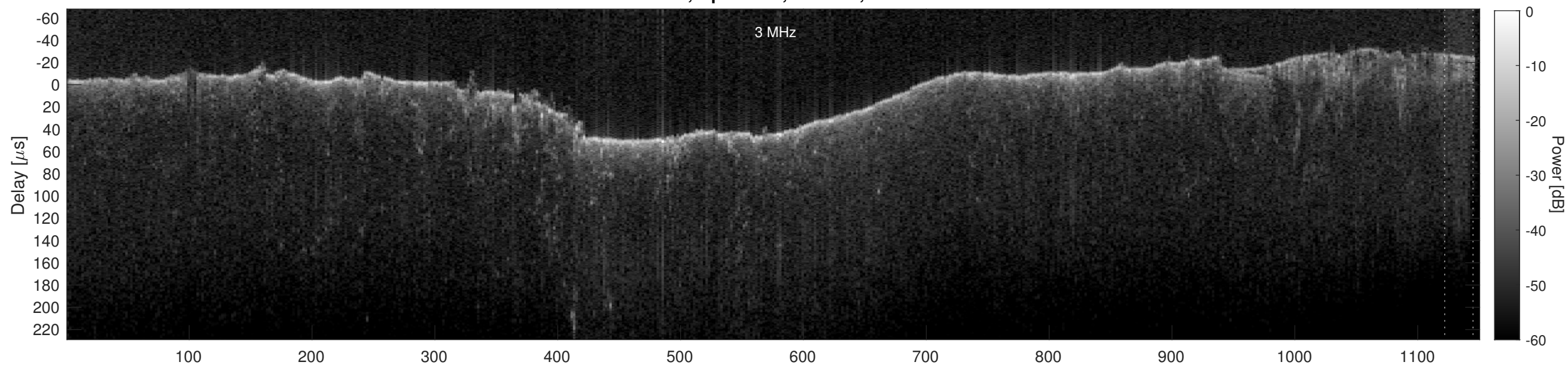
Orbit 11089, Cluttergram
