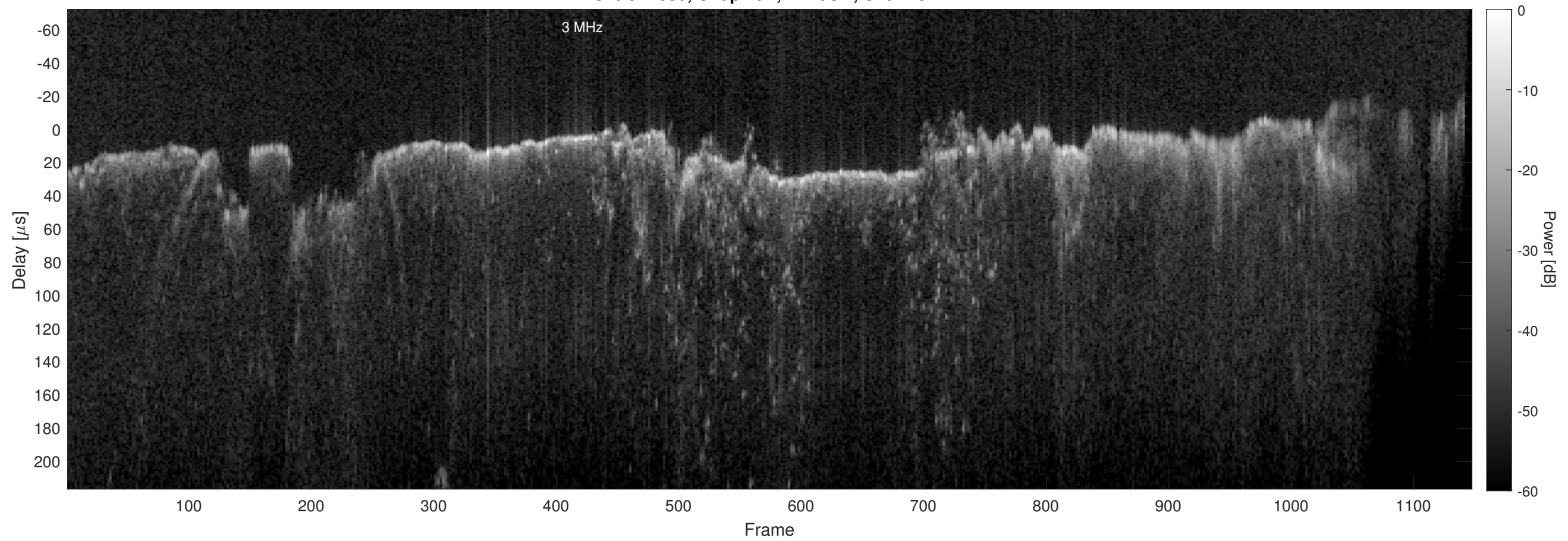
Orbit 11090, Chapman, Window, Channel 2
