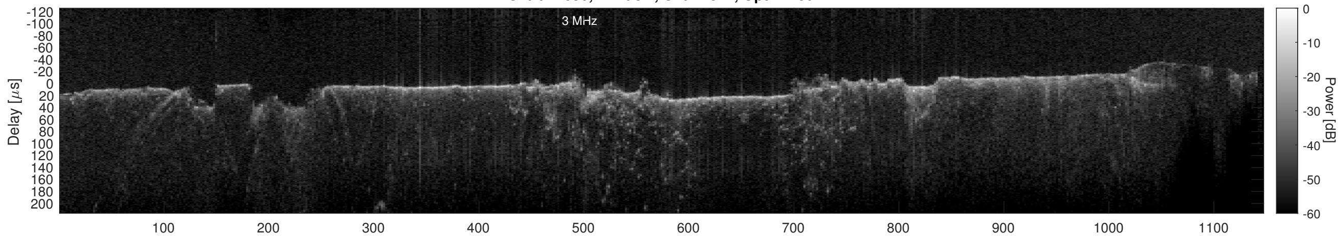
Orbit 11090, Cluttergram
