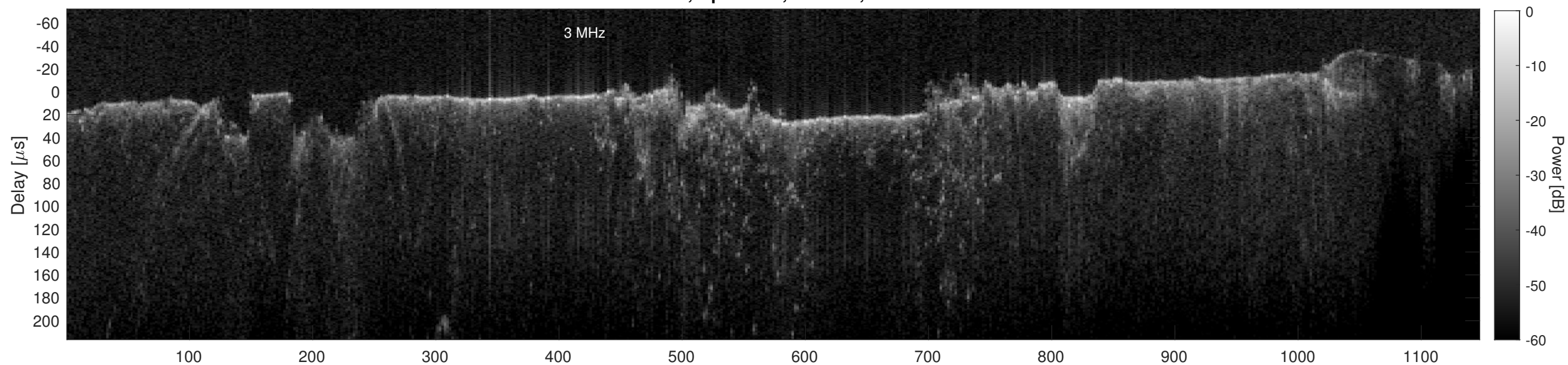
Orbit 11090, Cluttergram
