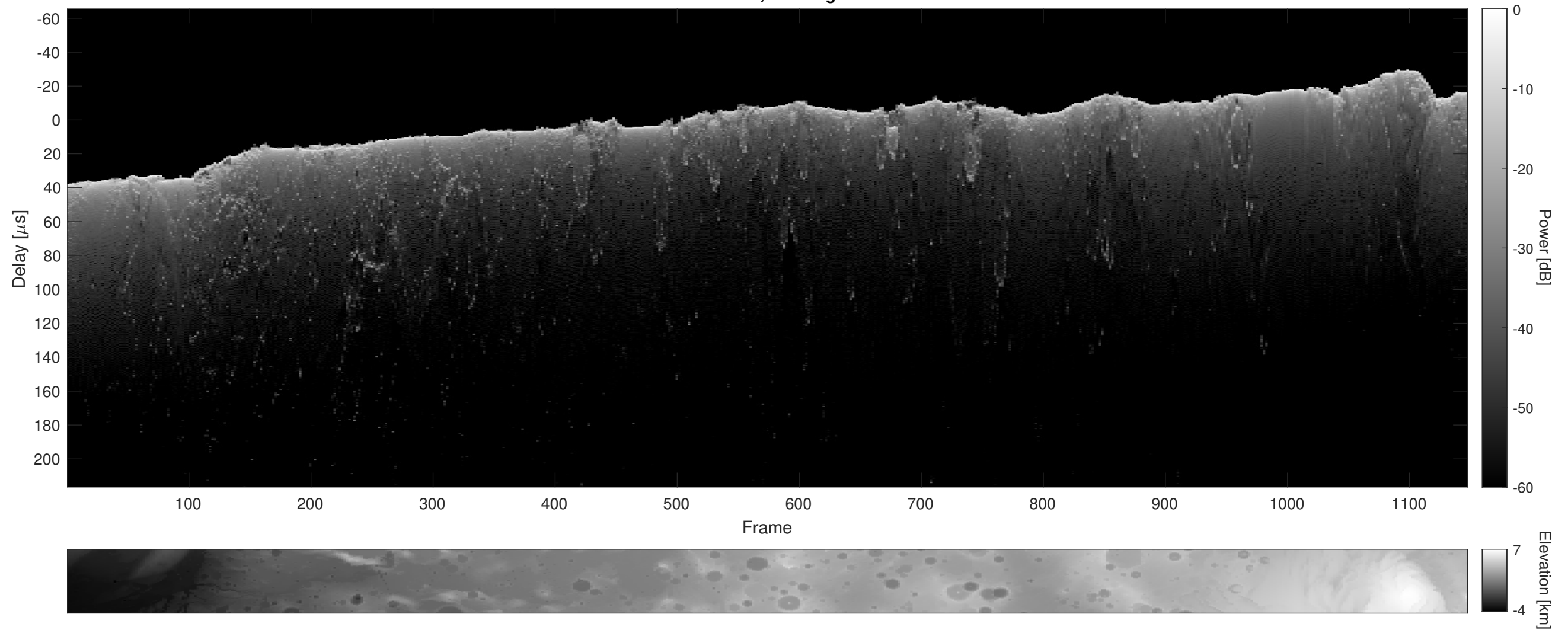
Orbit 11091, Cluttergram
