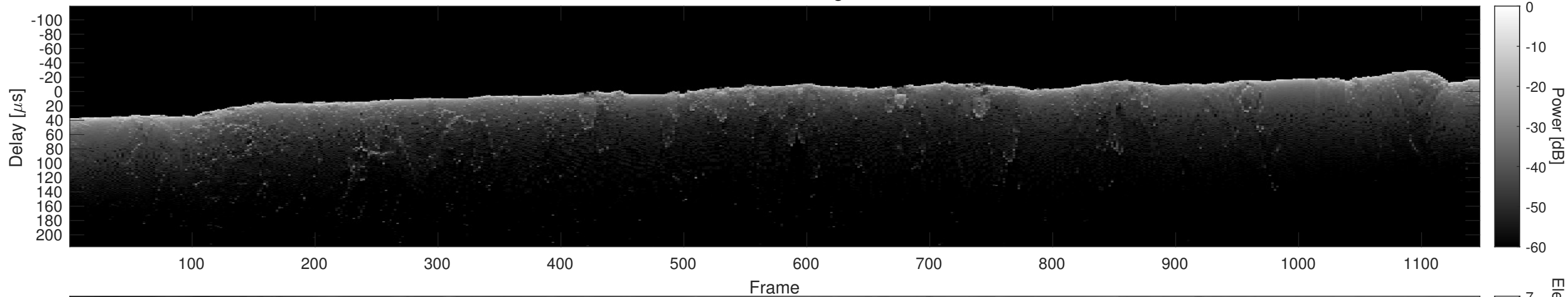
Orbit 11091, Cluttergram
