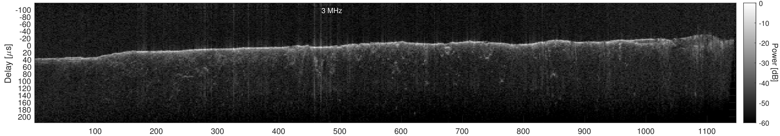
Orbit 11091, Cluttergram
