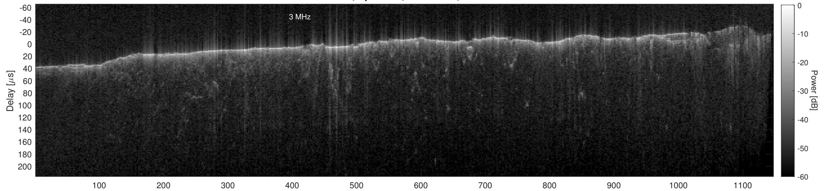
Orbit 11091, Cluttergram
