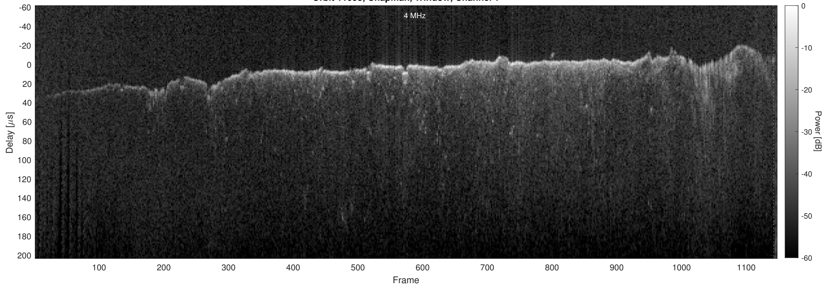
Orbit 11093, Chapman, Window, Channel 2
