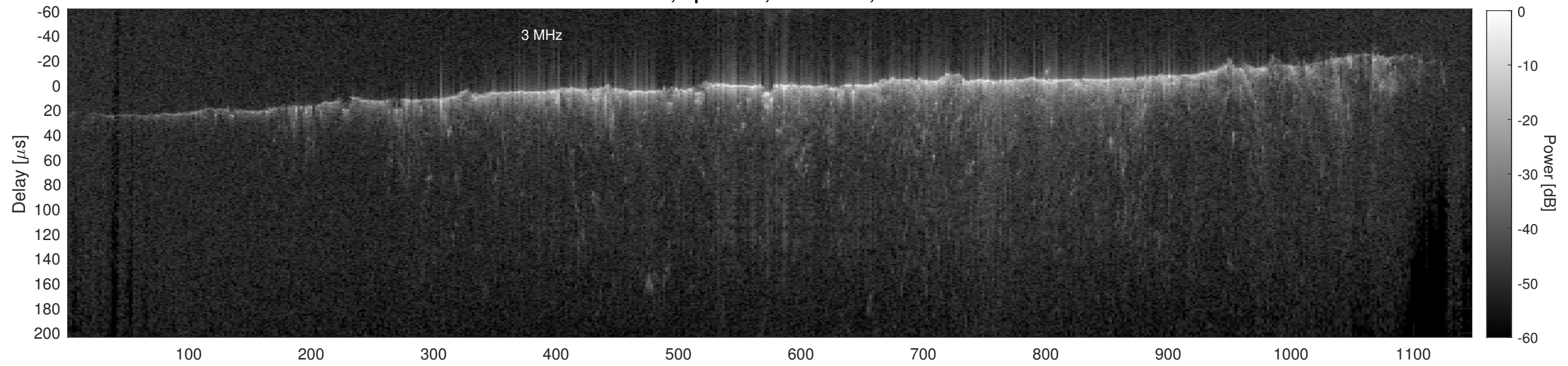
Orbit 11093, Cluttergram
