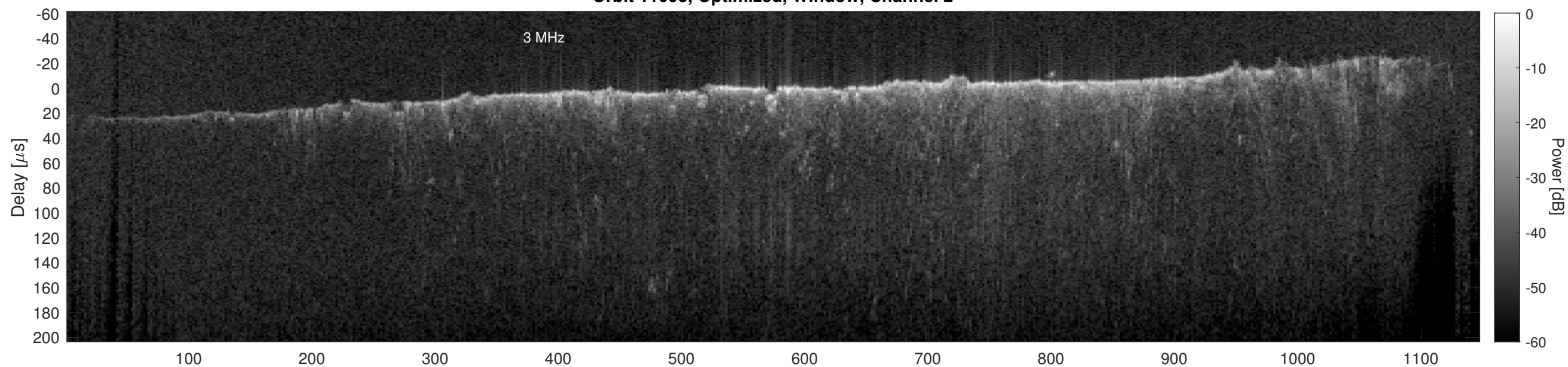
Orbit 11093, Cluttergram
