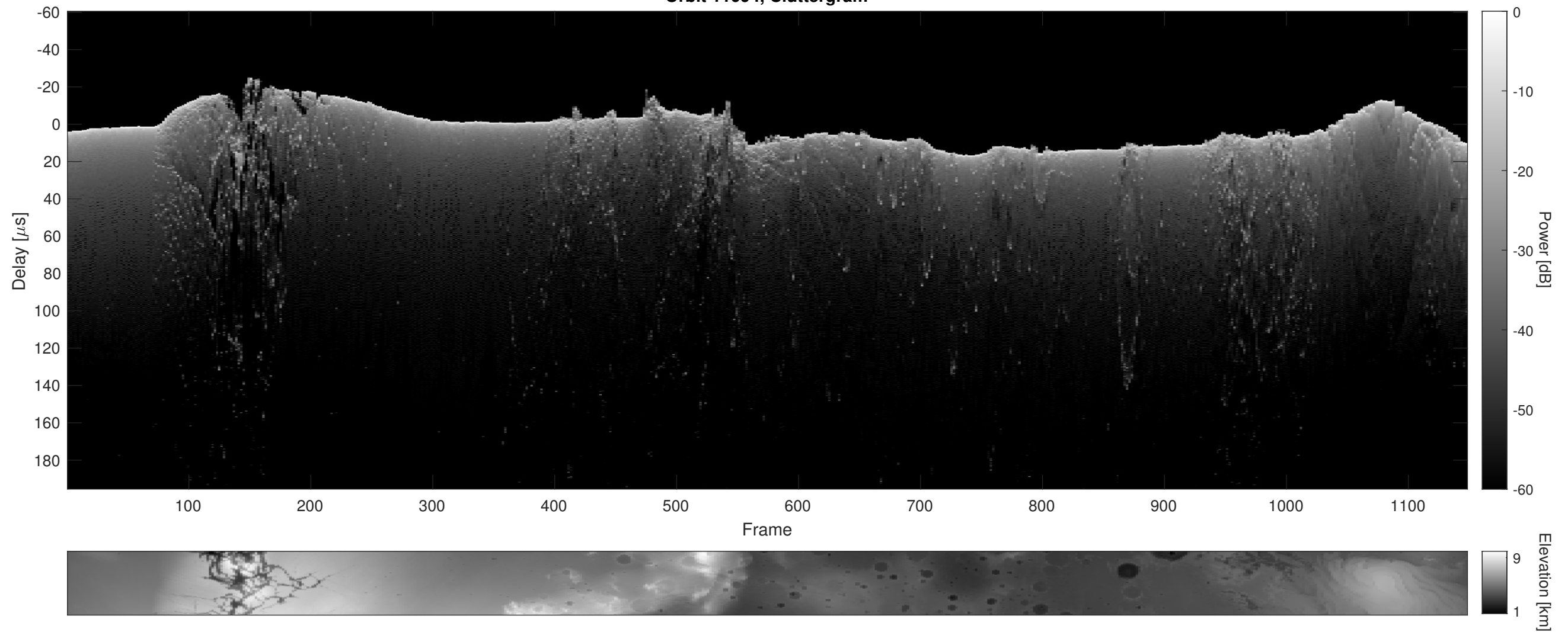
Orbit 11094, Cluttergram
