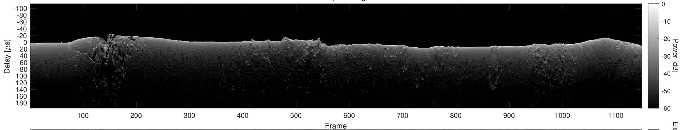
Orbit 11094, Cluttergram
