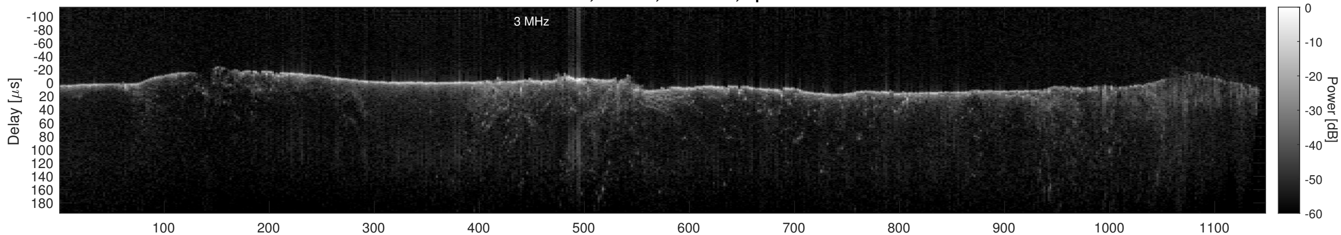
Orbit 11094, Cluttergram
