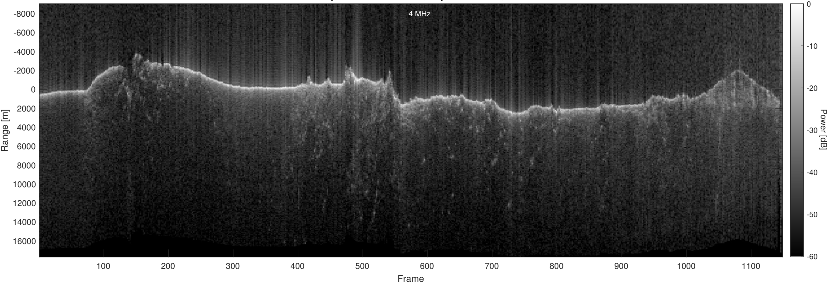
Orbit 11094, Optimized, No Window, Depth-Corrected, Channel 2
