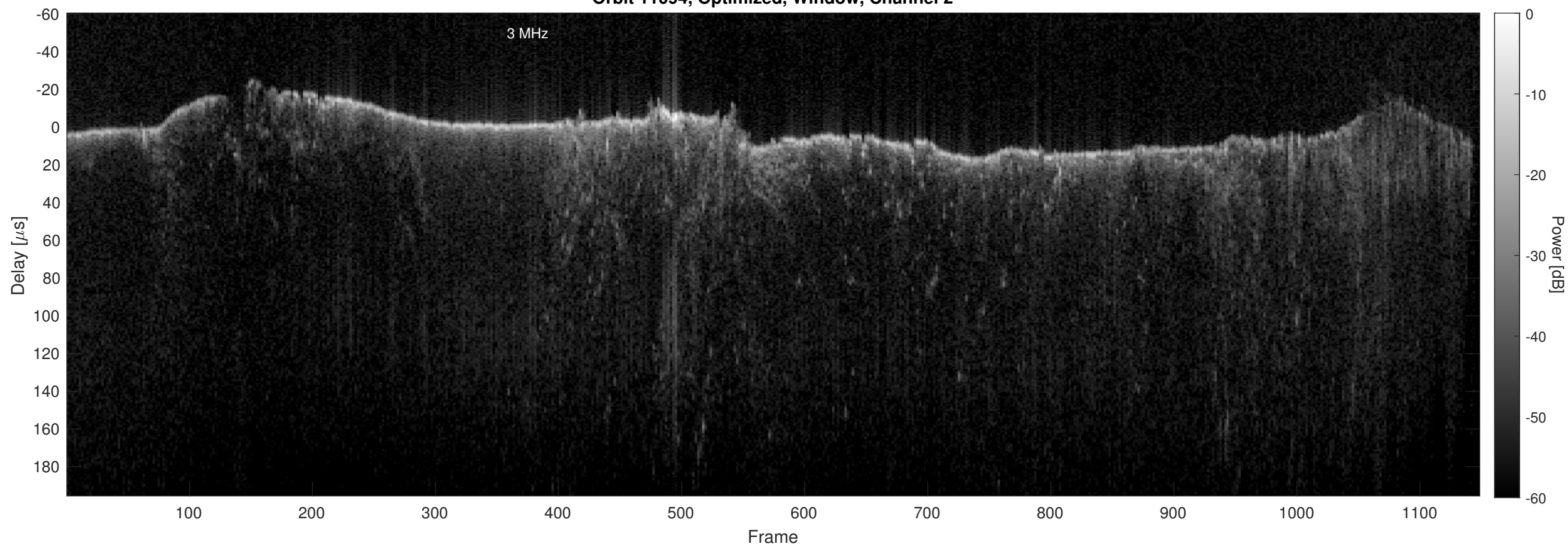
Orbit 11094, Optimized, Window, Channel 2
