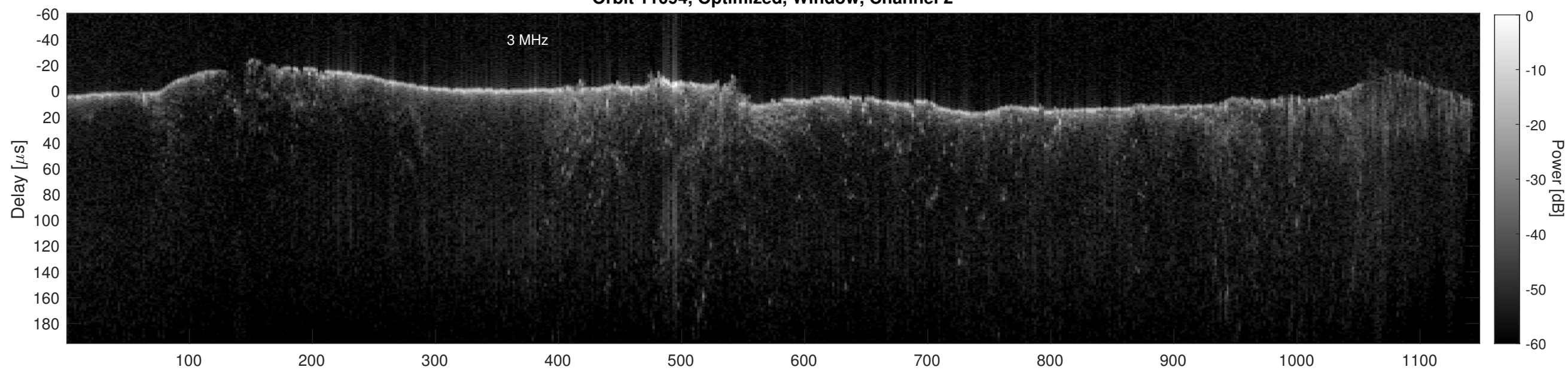
Orbit 11094, Cluttergram
