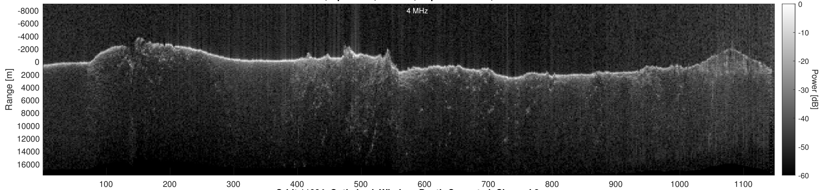
Orbit 11094, Optimized, Window, Depth-Corrected, Channel 2
