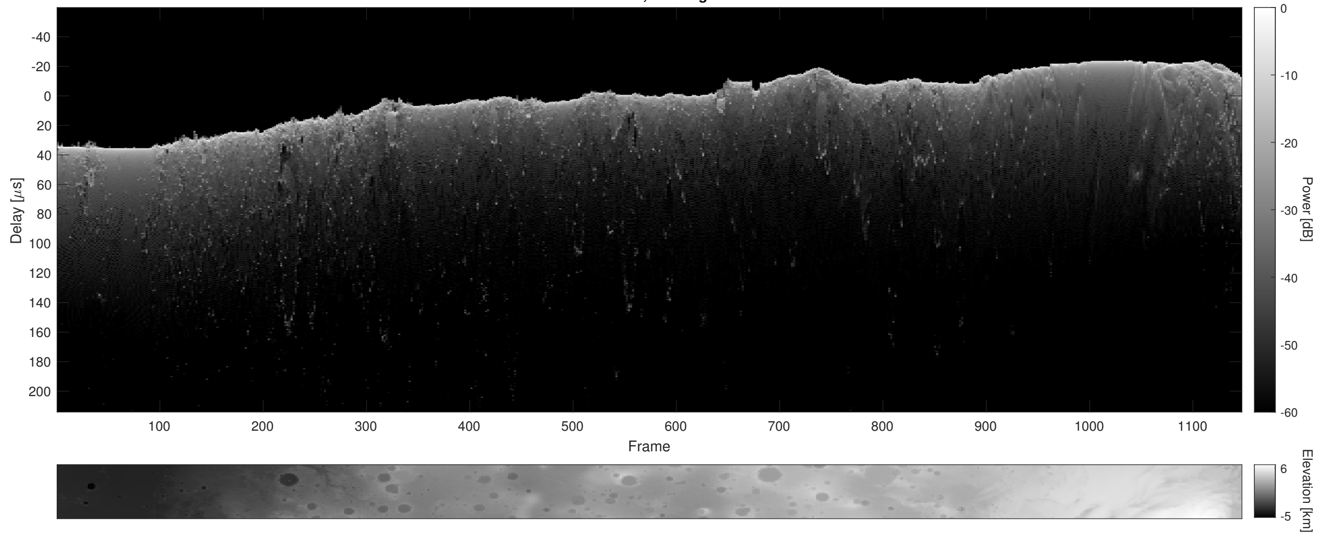
Orbit 11095, Cluttergram
