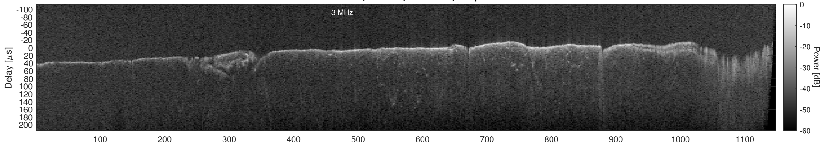
Orbit 11095, Window, Channel 2, Optimized
