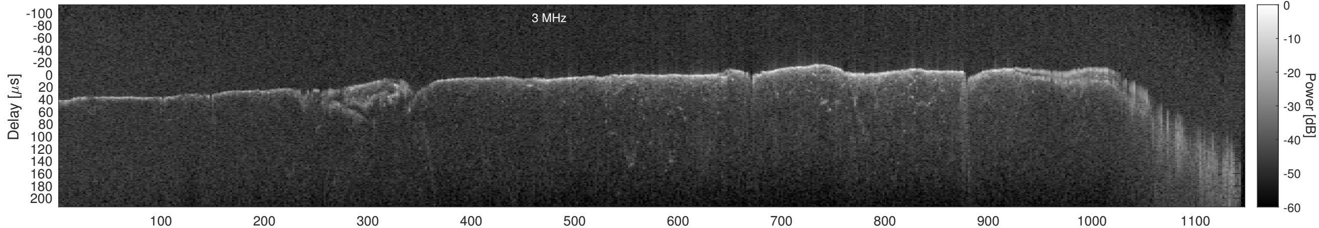
Orbit 11095, Window, Channel 2, Chapman
