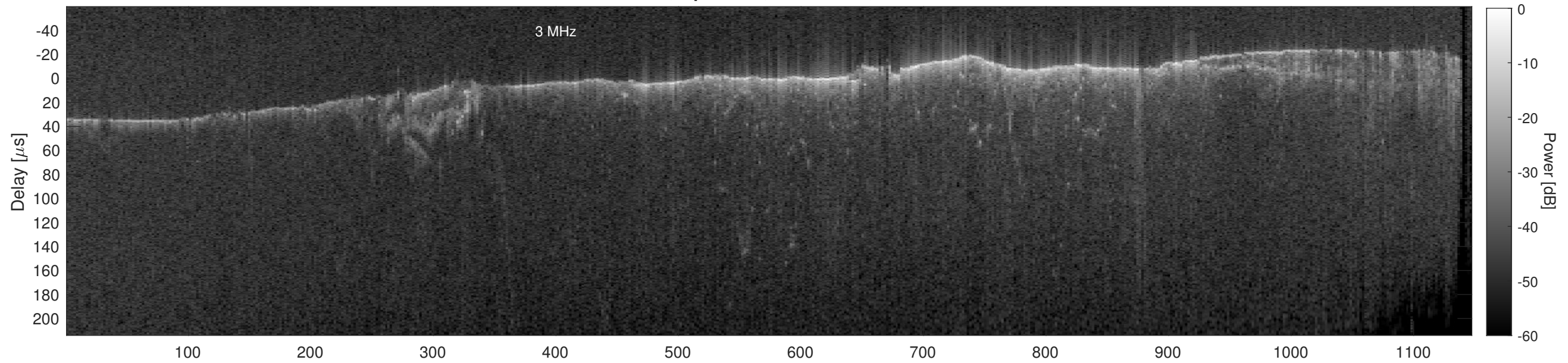
Orbit 11095, Cluttergram
