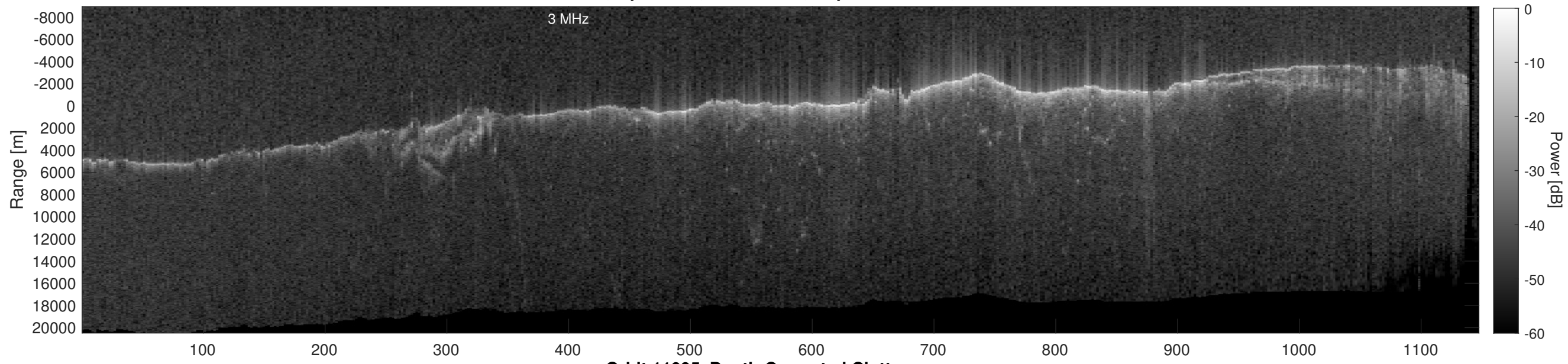
Orbit 11095, Depth-Corrected Cluttergram
