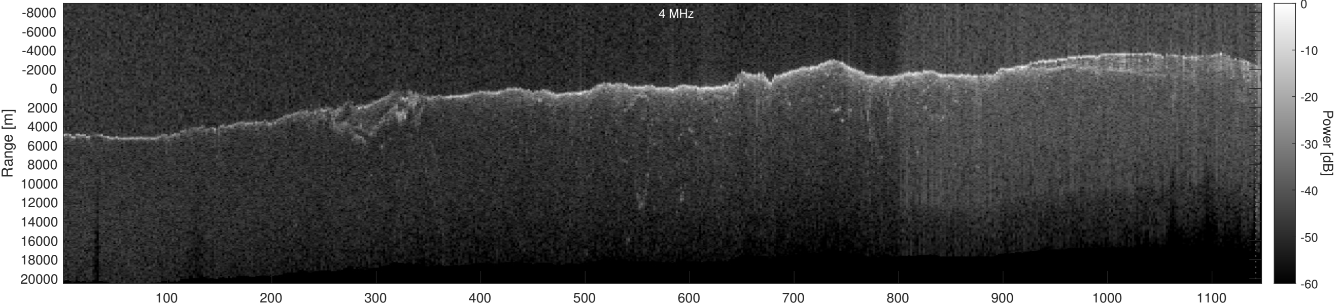
Orbit 11095, Optimized, Window, Depth-Corrected, Channel 2
