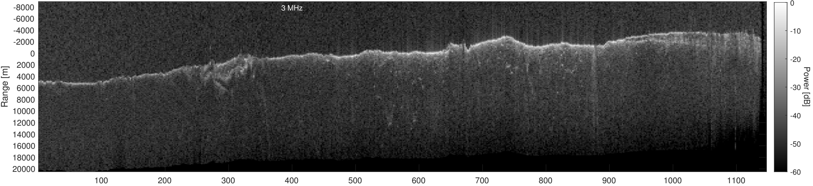
Orbit 11095, Depth-Corrected Cluttergram
