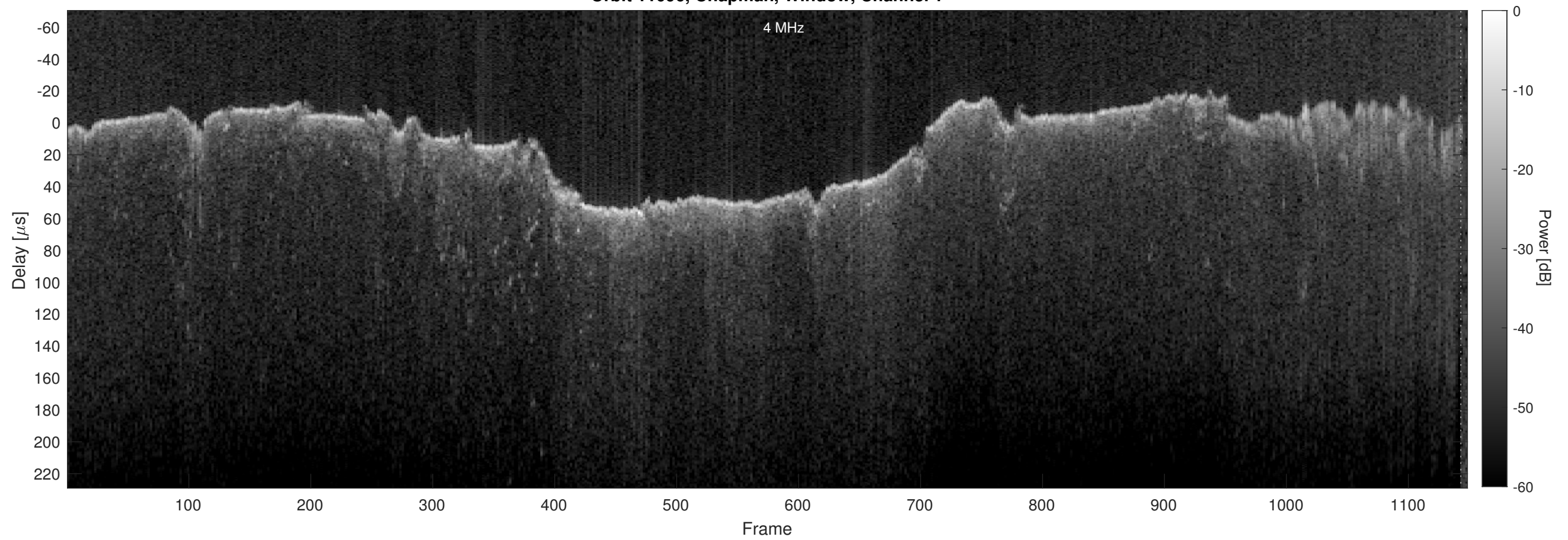
Orbit 11096, Chapman, Window, Channel 2
