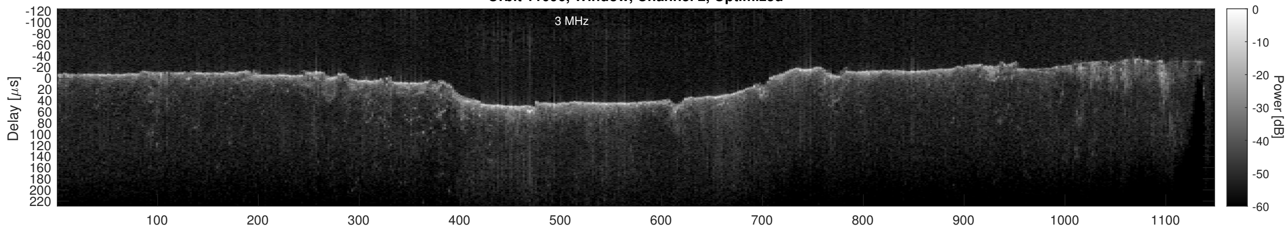
Orbit 11096, Cluttergram
