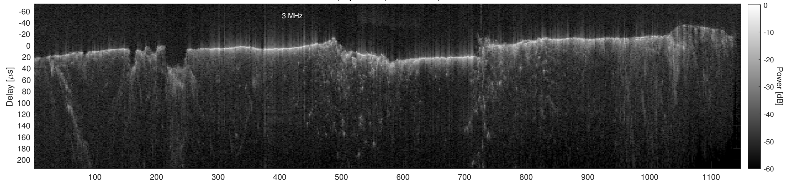
Orbit 11097, Cluttergram
