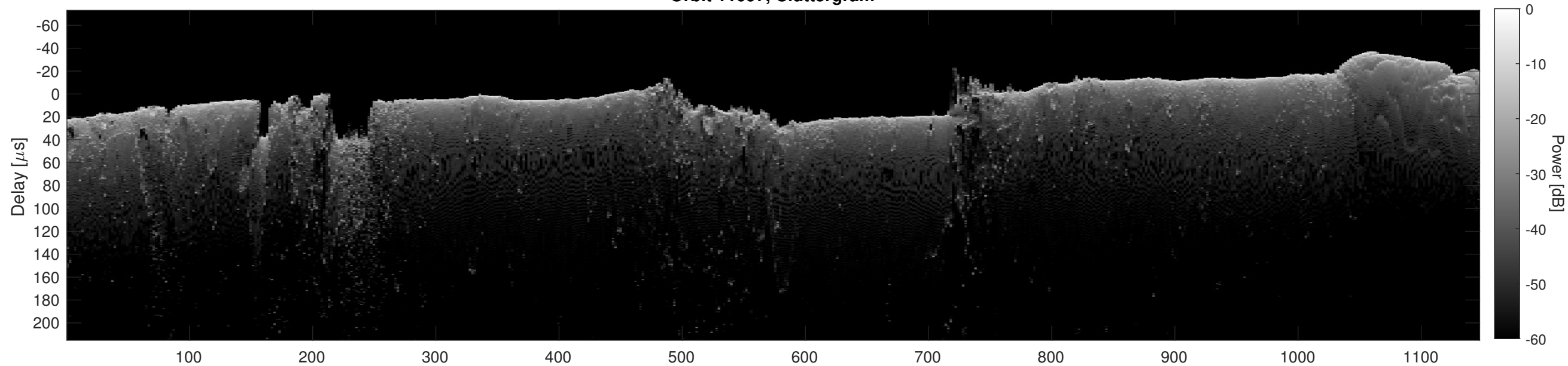
Orbit 11097, Cluttergram
