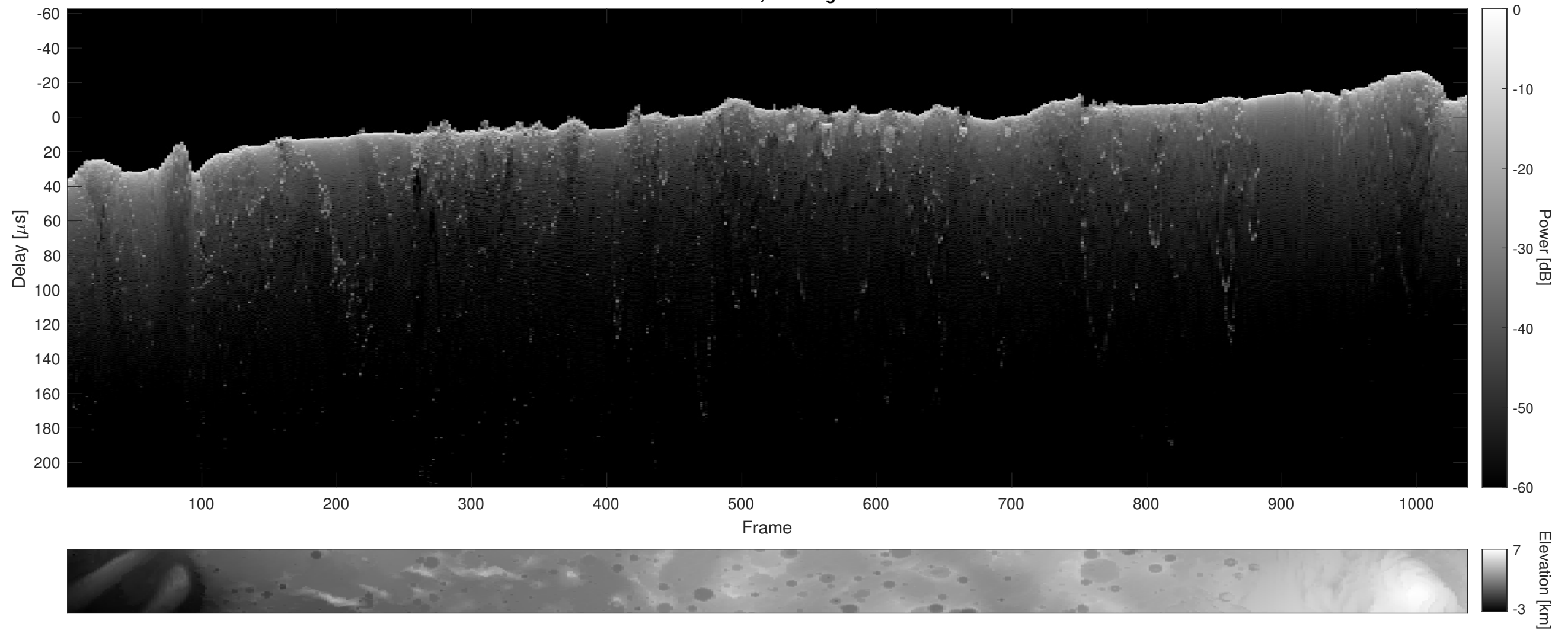
Orbit 11098, Cluttergram
