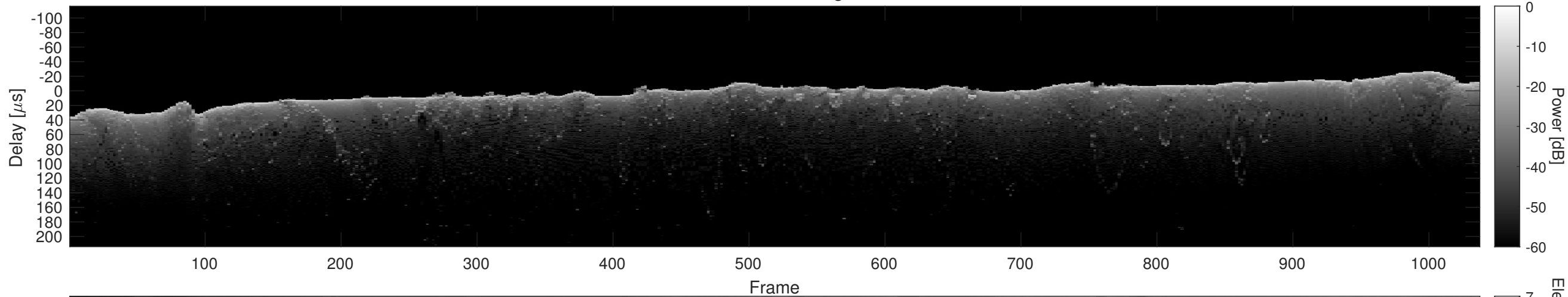
Orbit 11098, Cluttergram
