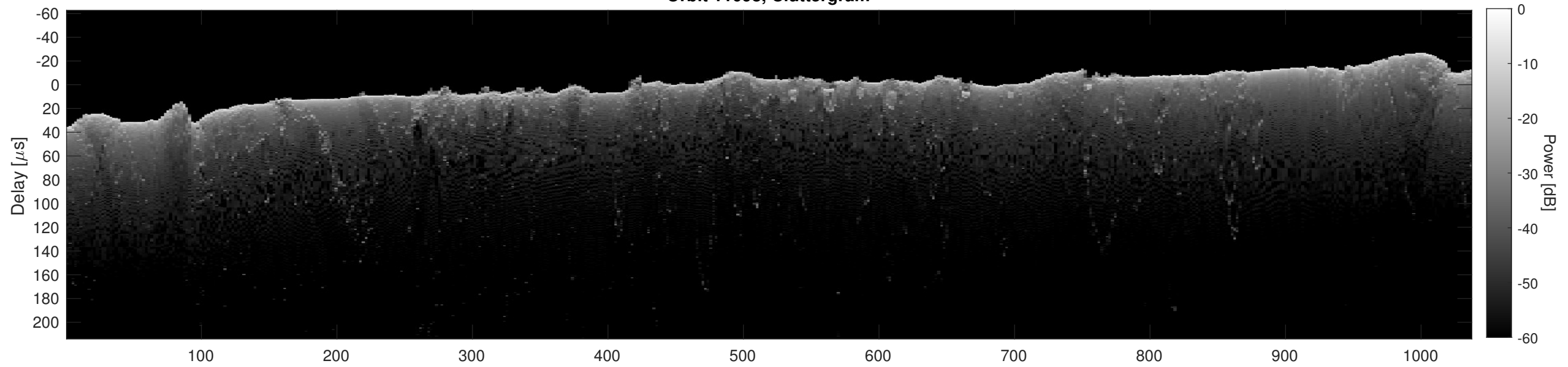
Orbit 11098, Cluttergram
