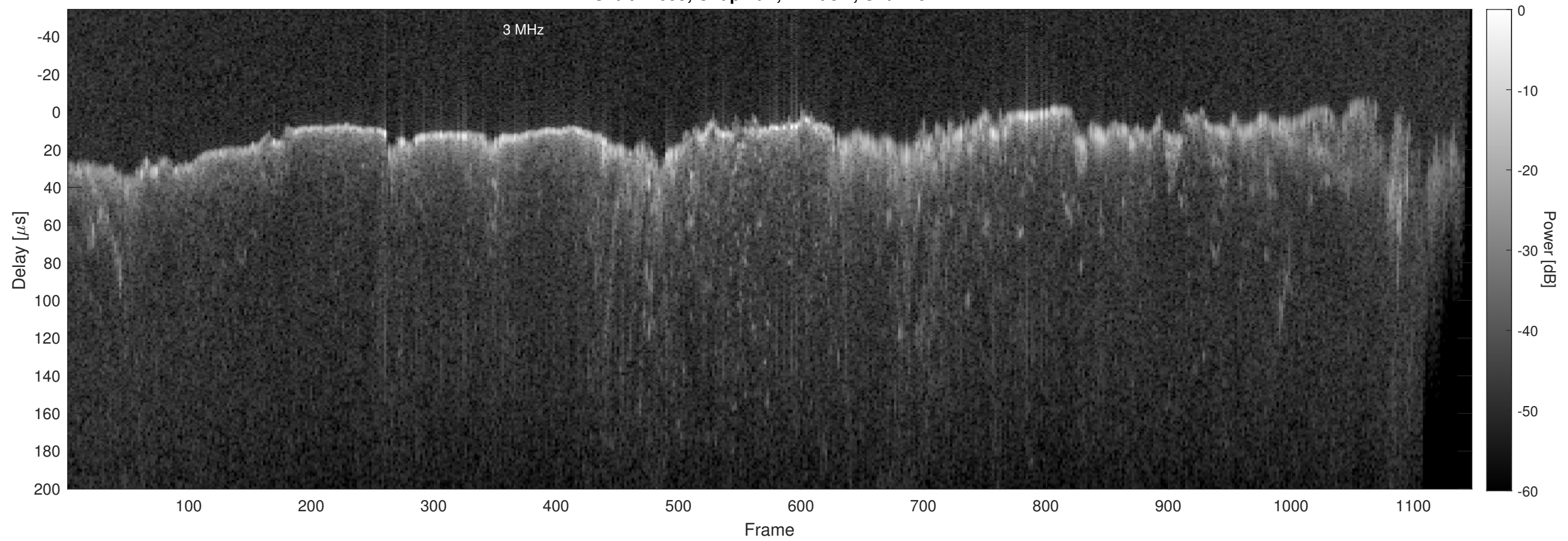
Orbit 11099, Chapman, Window, Channel 2
