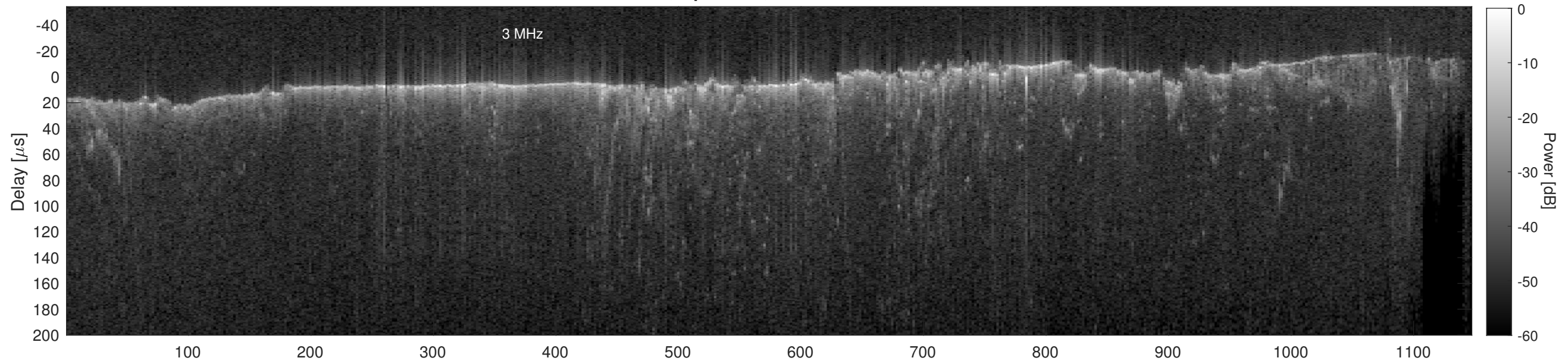
Orbit 11099, Cluttergram
