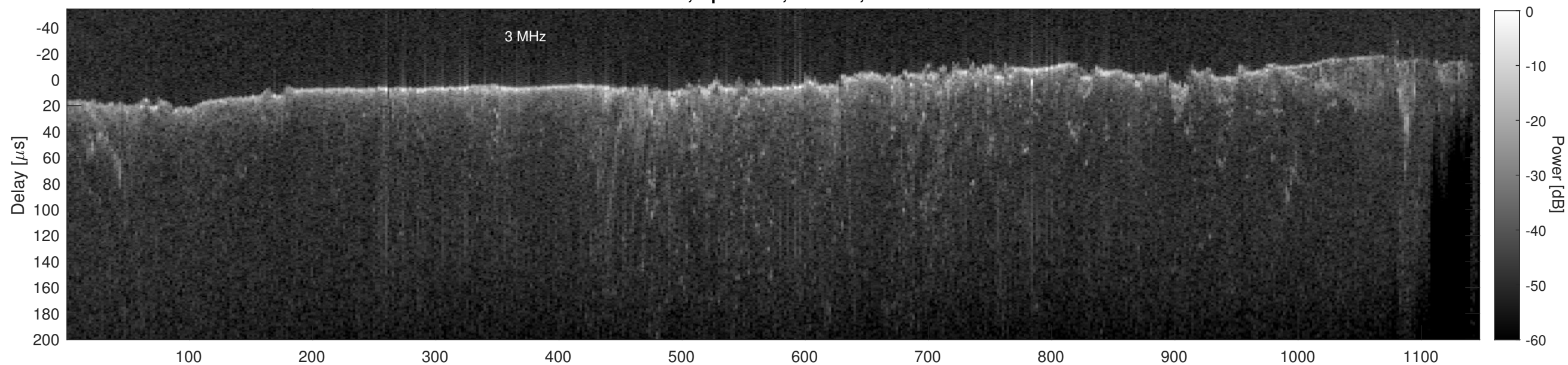
Orbit 11099, Cluttergram
