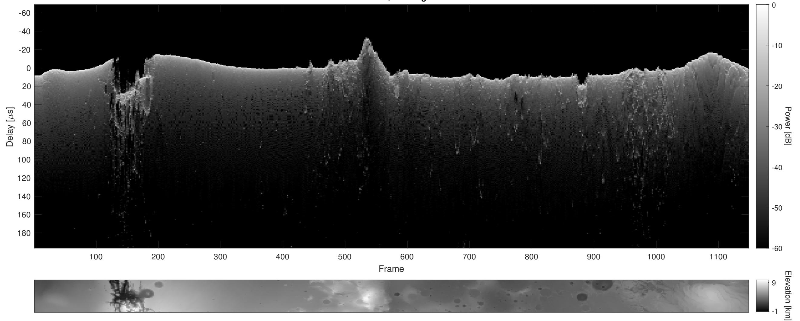
Orbit 11101, Cluttergram
