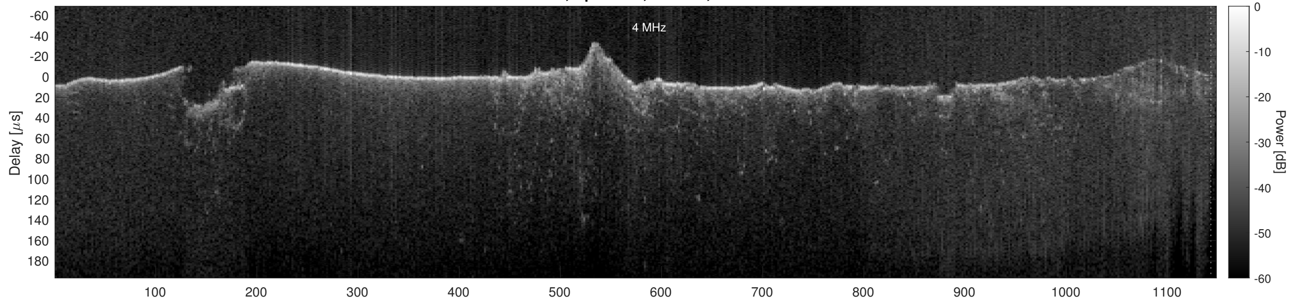
Orbit 11101, Optimized, Window, Channel 2
