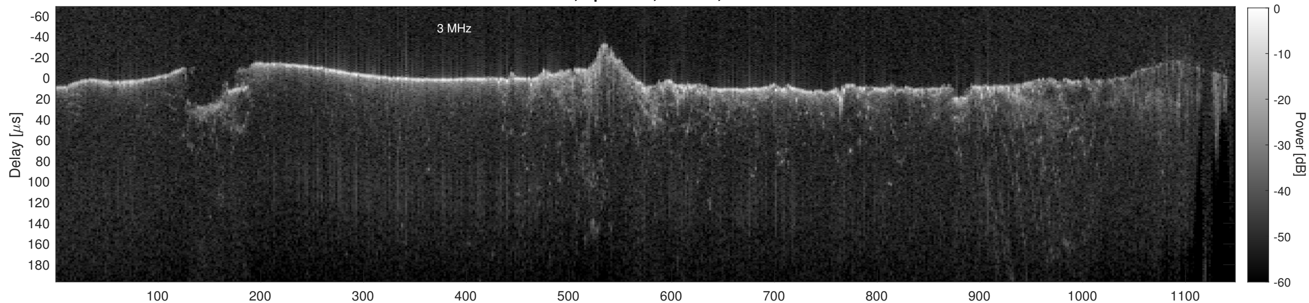
Orbit 11101, Cluttergram
