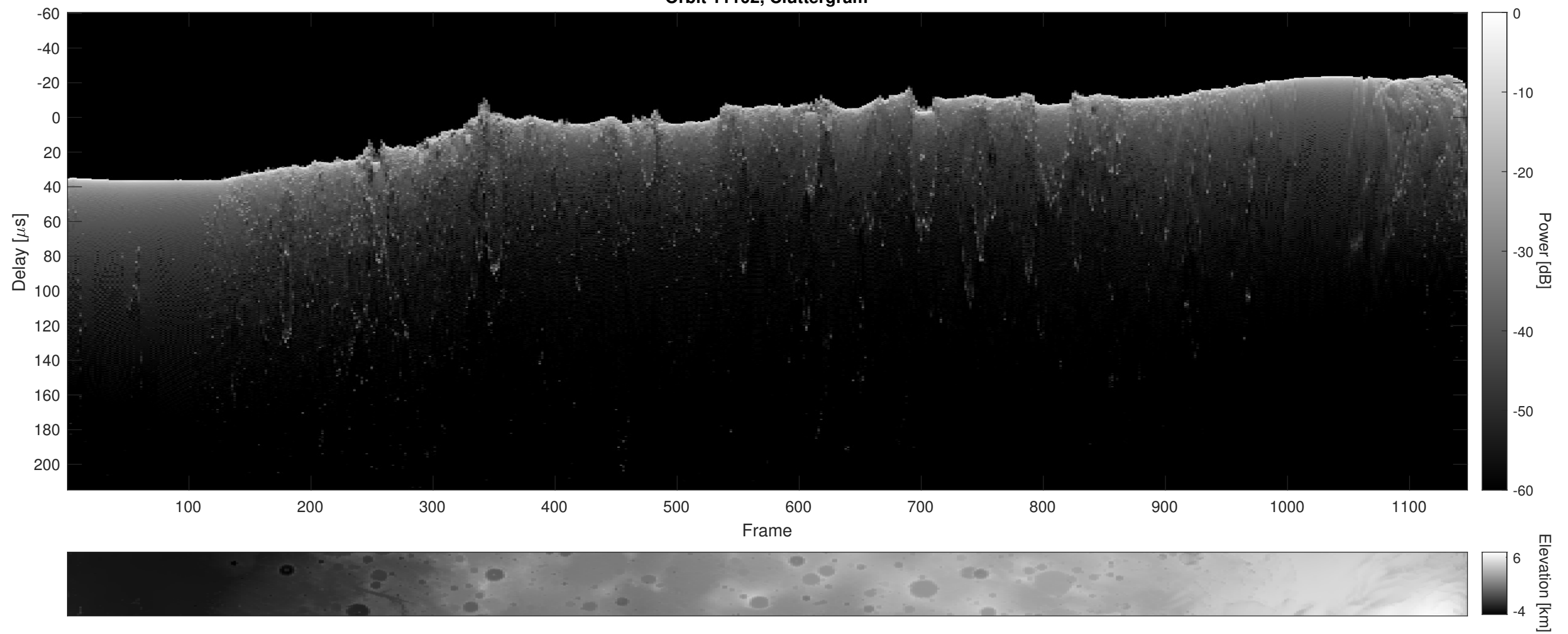
Orbit 11102, Cluttergram
