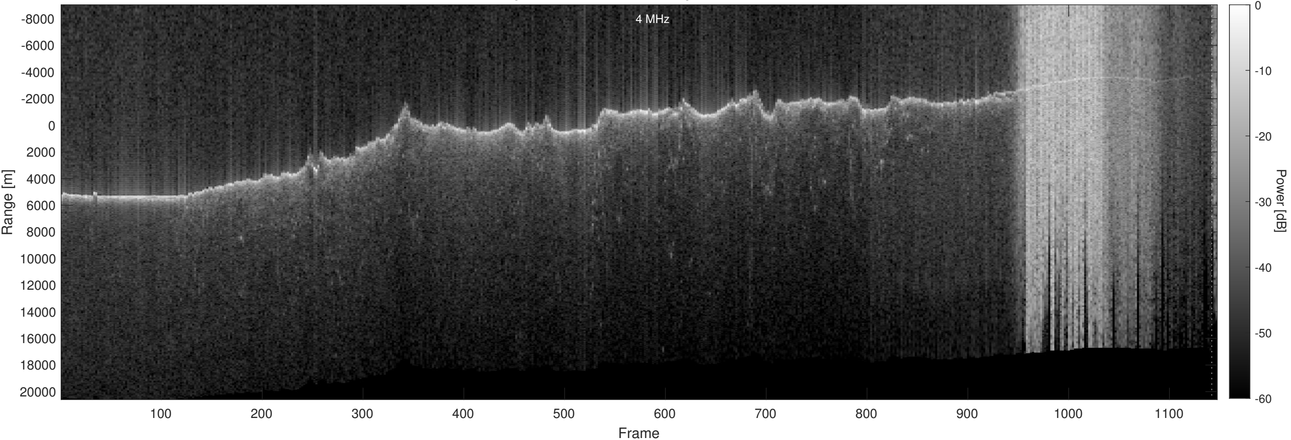
Orbit 11102, Optimized, No Window, Depth-Corrected, Channel 2
