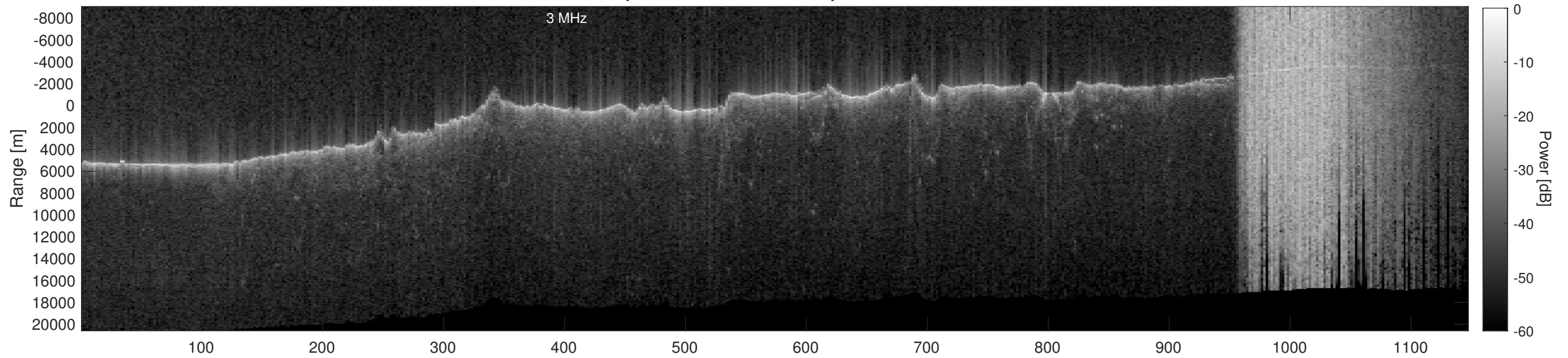
Orbit 11102, Depth-Corrected Cluttergram
