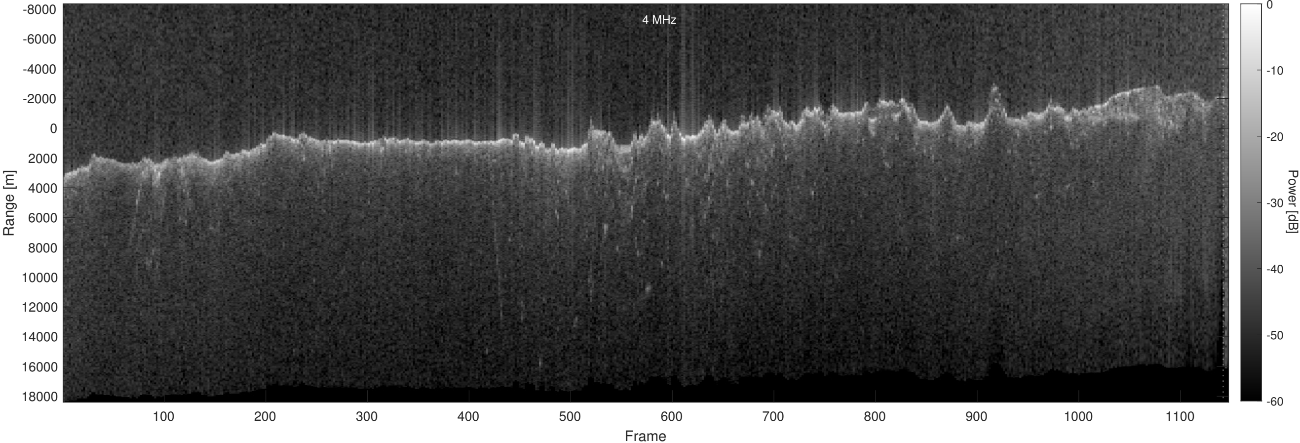
Orbit 11106, Optimized, No Window, Depth-Corrected, Channel 2
