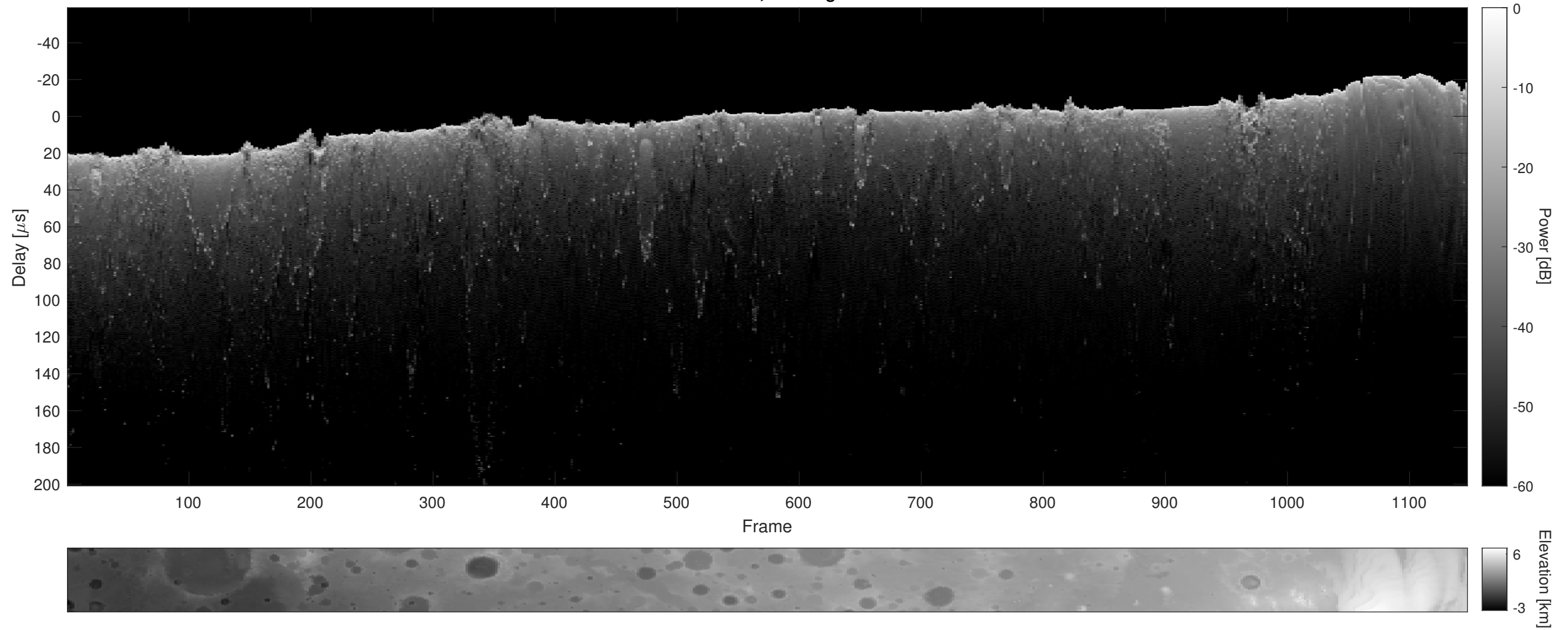
Orbit 11107, Cluttergram
