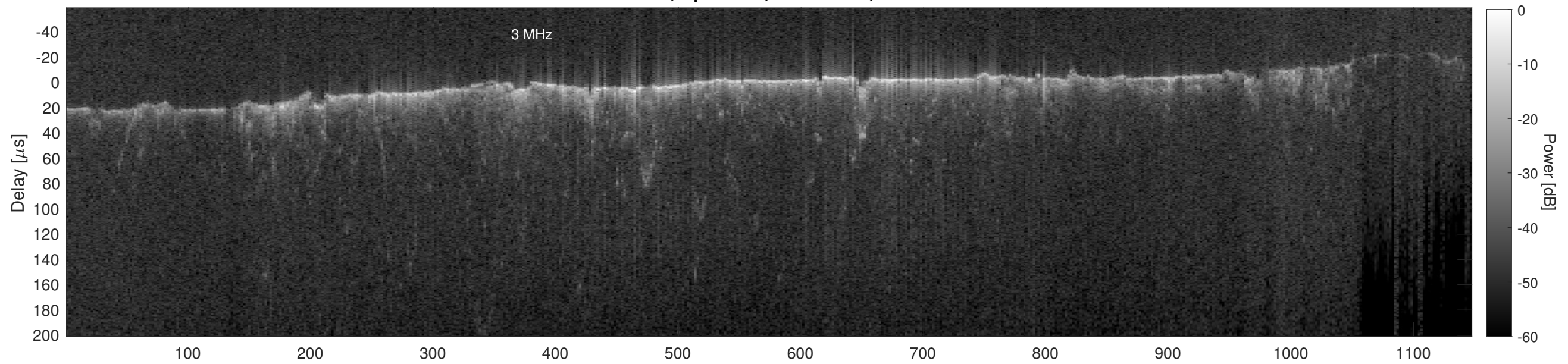
Orbit 11107, Cluttergram
