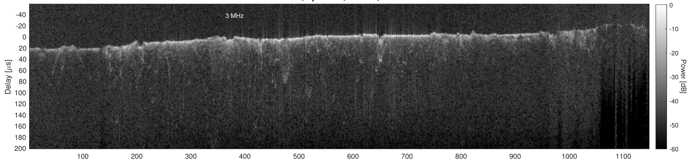
Orbit 11107, Cluttergram
