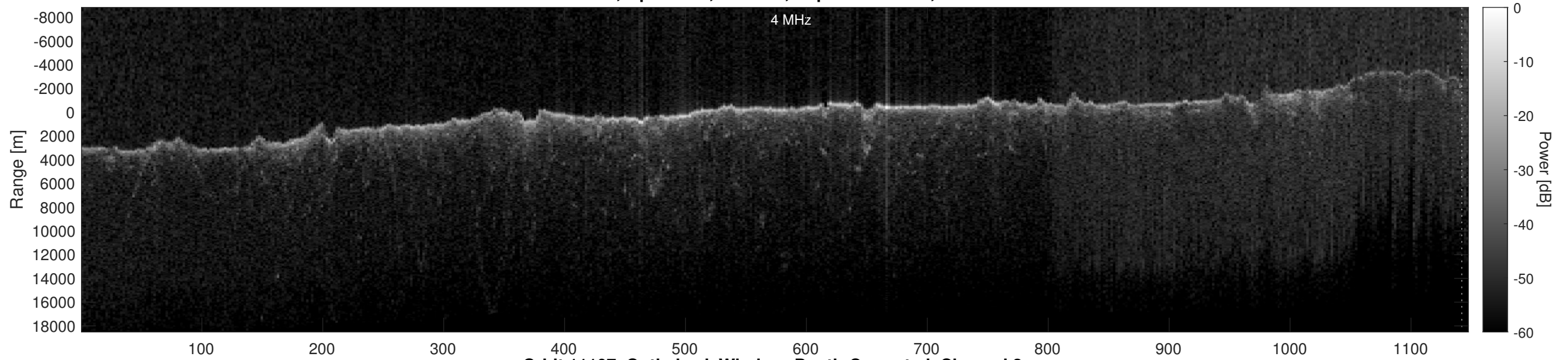
Orbit 11107, Optimized, Window, Depth-Corrected, Channel 2
